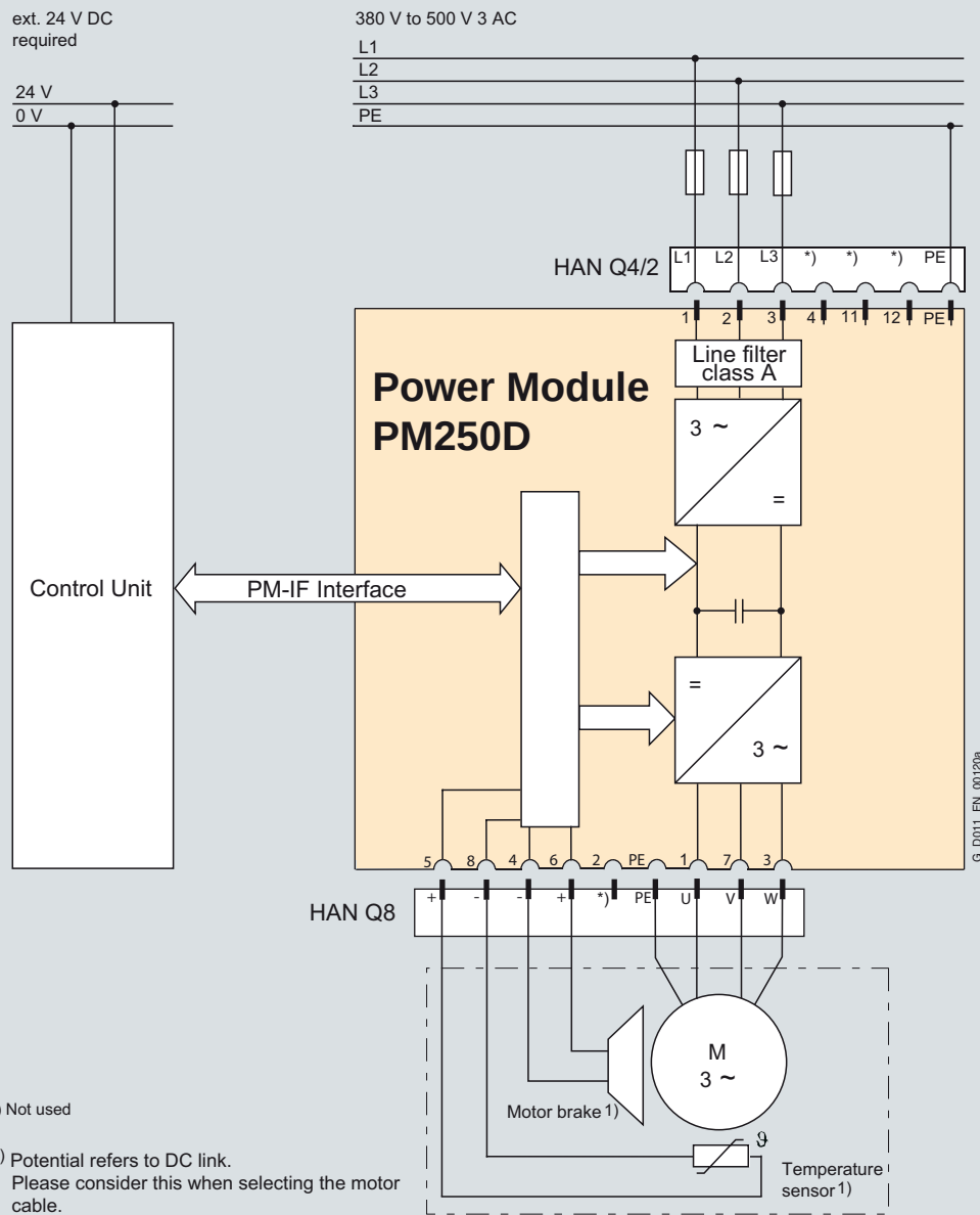
Connection diagram for PM250D Power Module with integrated class A line filter
