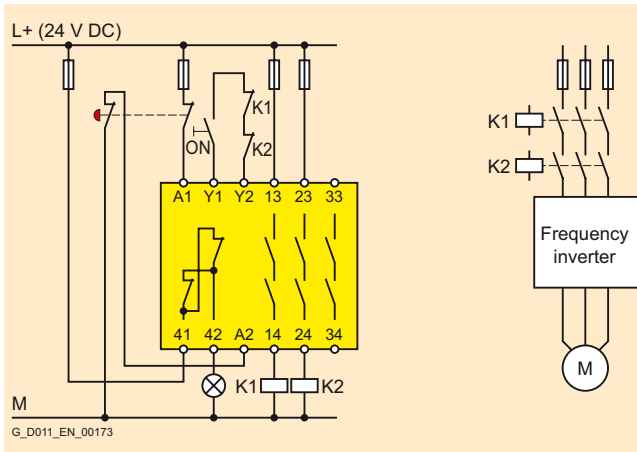
Conventional wiring
