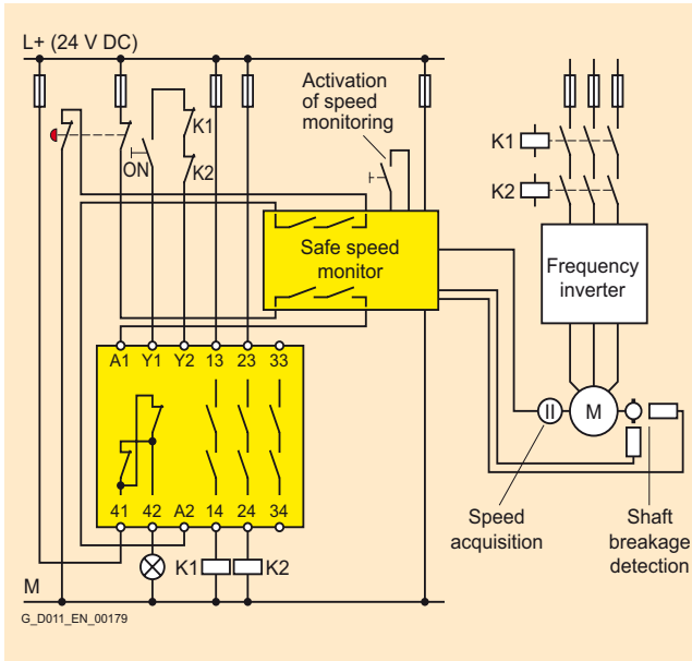
Conventional wiring
