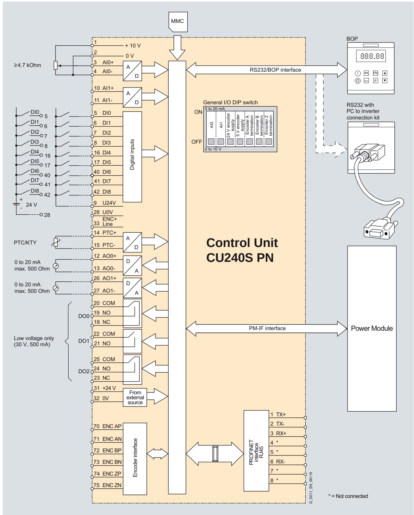
CU240S PN Control Unit connection diagram
