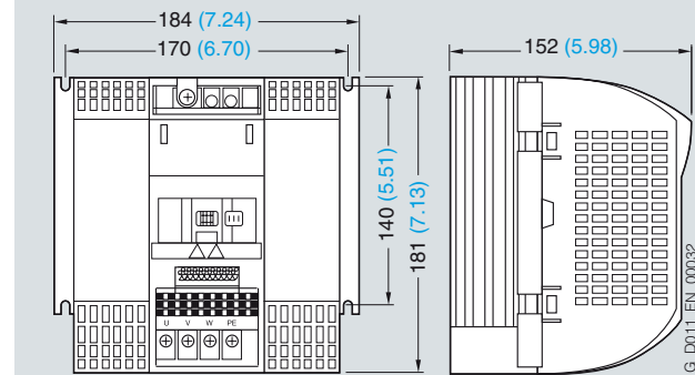
Inverter frame size FSC; 2.2 kW to 3.0 kW (3.0 hp to 4.0 hp)
