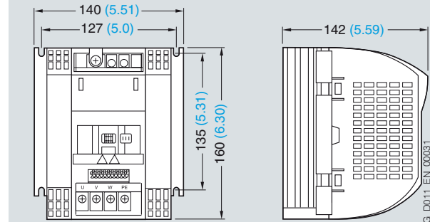
Inverter frame size FSB; 1.1 kW to 1.5 kW (1.5 hp to 2.0 hp)
