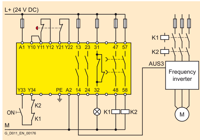
Conventional wiring
